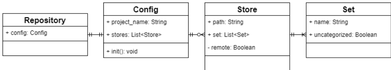
Figure 4: A UML diagram of the CrossDoc repository submodules.
