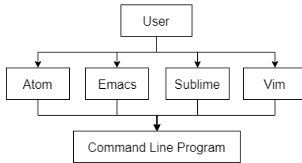
Figure 5: An architectural diagram of the text editor plugin interaction flow.
