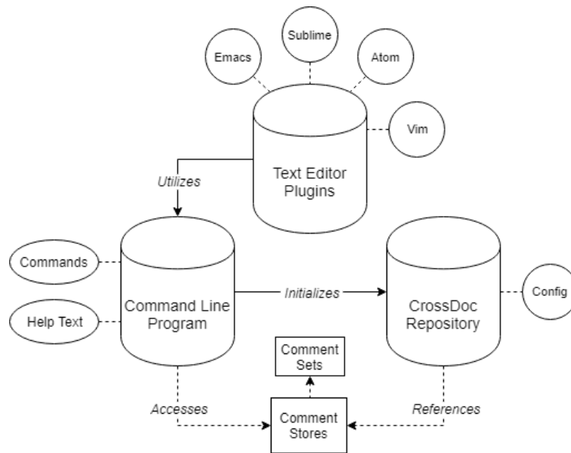
Figure 3: A high-level diagram of the CrossDoc module architecture.
